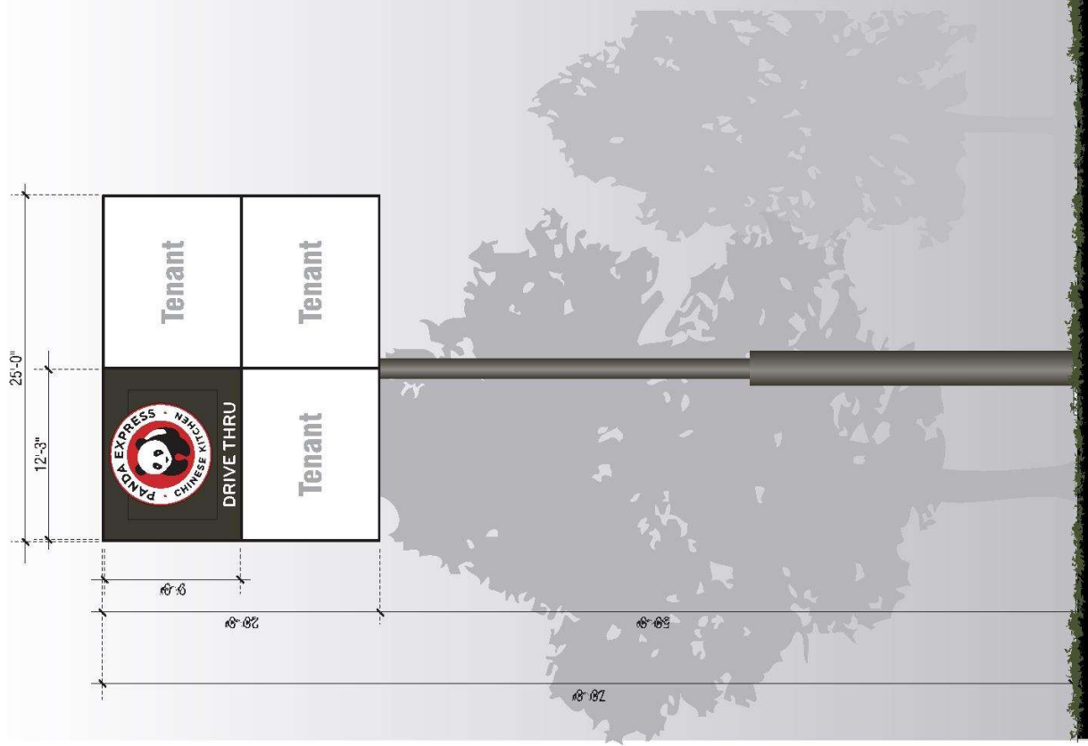
Z1 DOUBLE FACE ILLUMINATED TENANT POLE SIGN Quantity: One (1) Required
