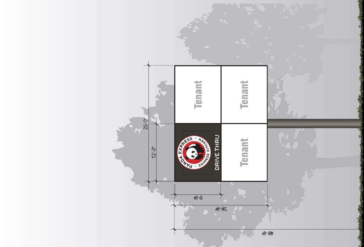
Z2 DOUBLE FACE ILLUMINATED TENANT POLE SIGN Quantity: One (1) Required
